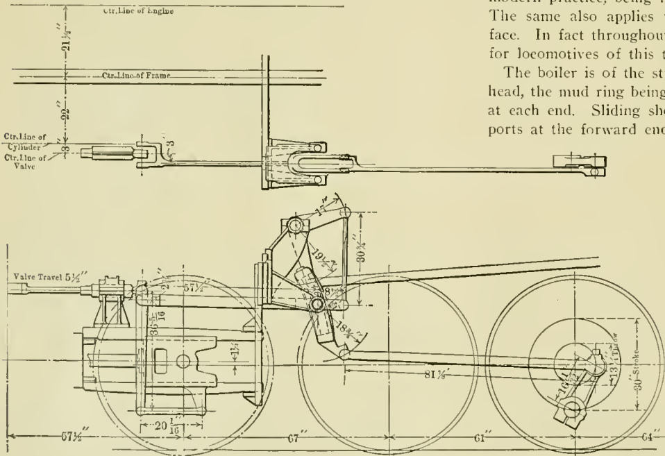
WALSCHAERT VALVE GEAR—C. N. O. & T. P. CONSOLIDATION LOCOMOTIVE.
